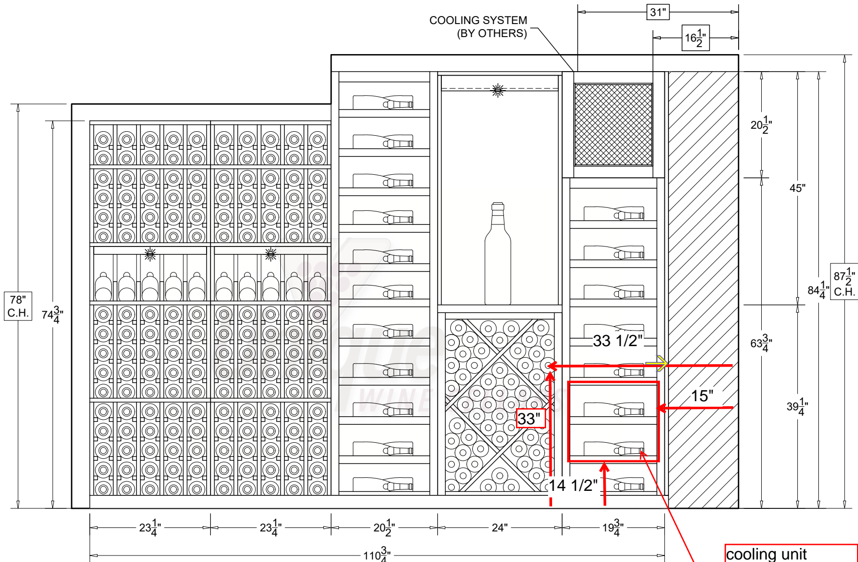
ELEVATION -A-
