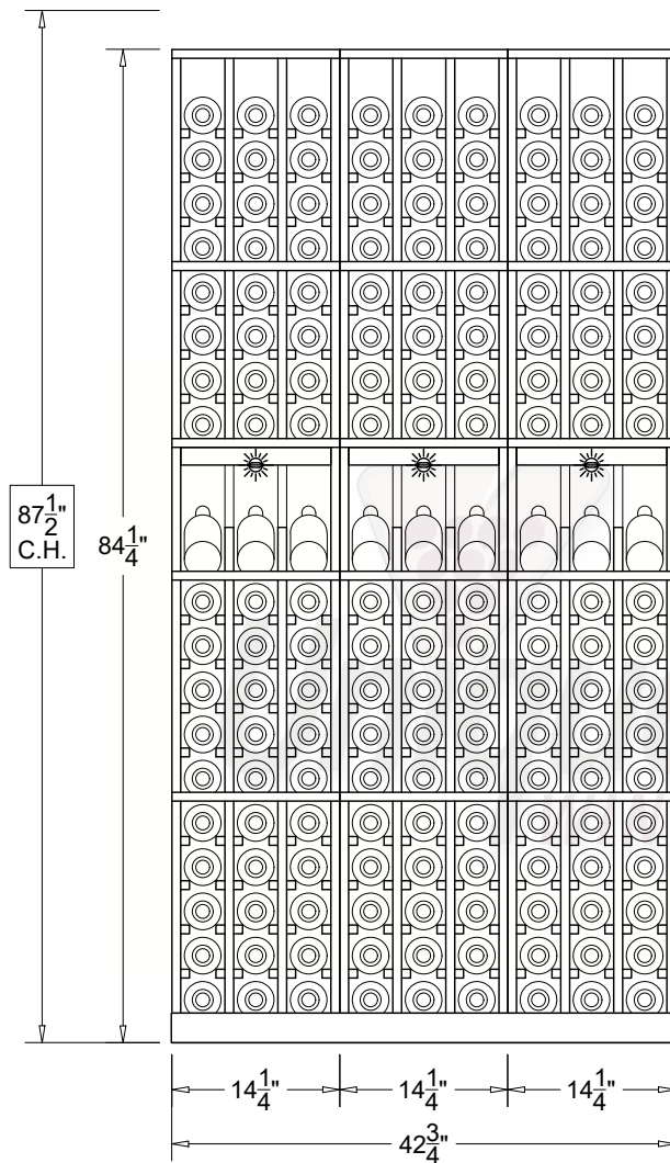
ELEVATION -B-
