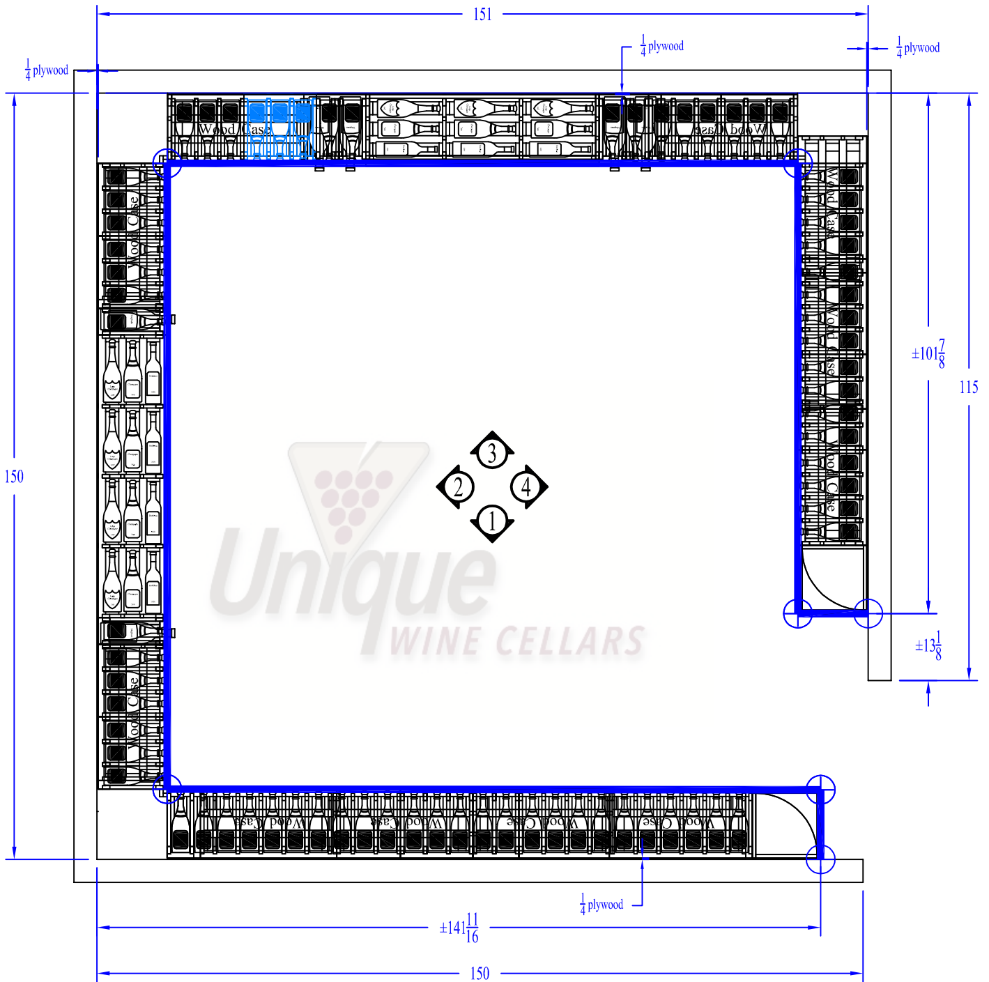
MOLDING PLAN ①
