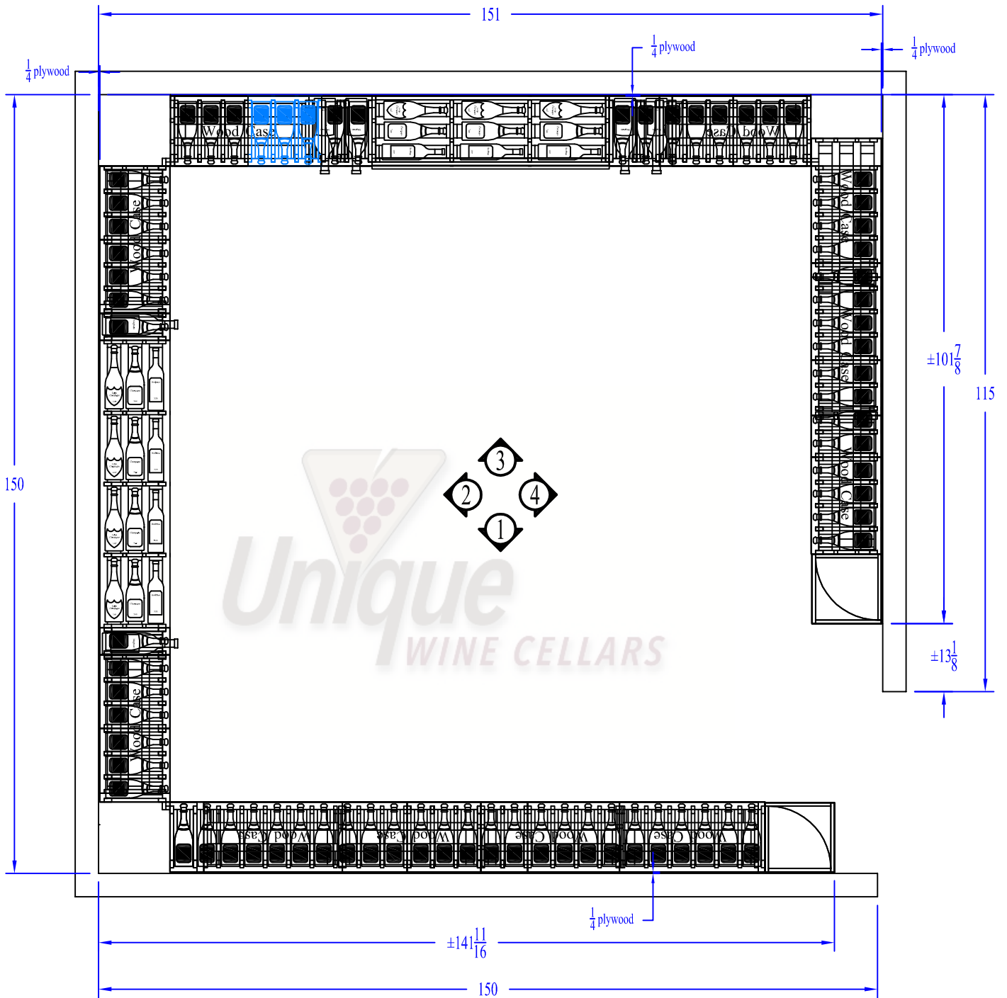
PLAN VIEW ①
