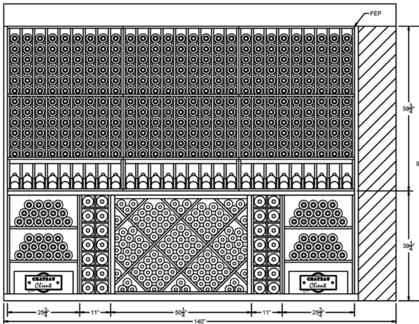
ELEVATION -A- (-C IS MIRROR)
