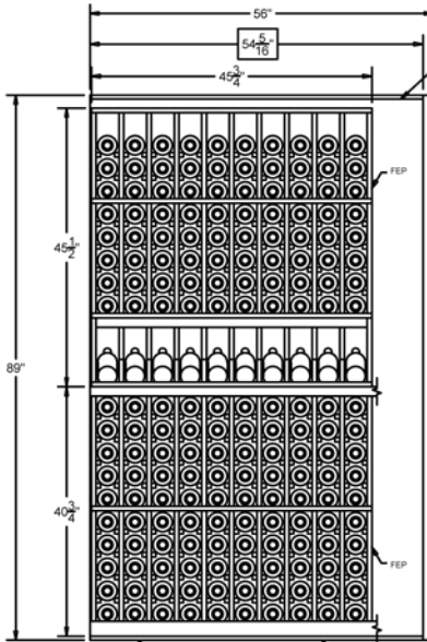
ELEVATION -A- (-E- IS MIRROR) INSTALLER TO SCRIBE RACKING ON ELEV. -E- AS NEEDED FOR COOLING SYSTEM
