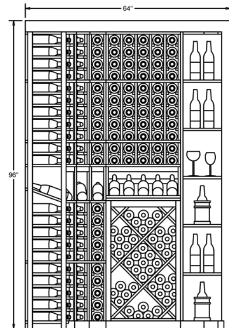
ELEVATION -B-
