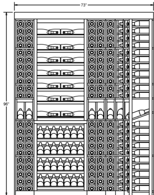
ELEVATION -A-
